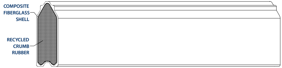
FIGURE 2 RUBBER FILLED
