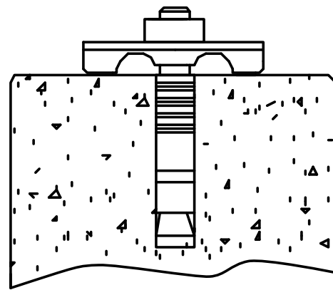
Base rail attachment hardware included.
